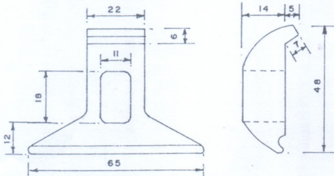
SUSPENSION CLAMP
