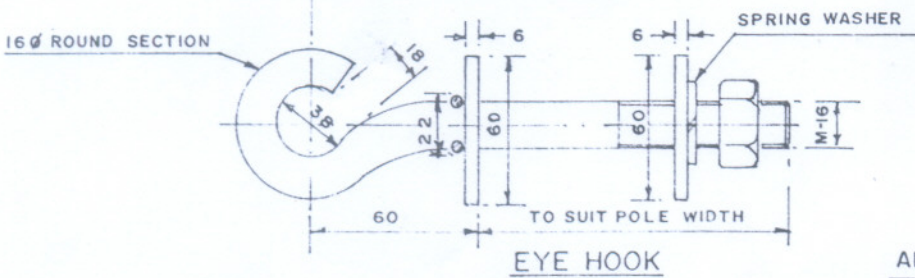
FIG. 1 DETAILS OF SUSPENSION CLAMP AND EYE HOOKS.
