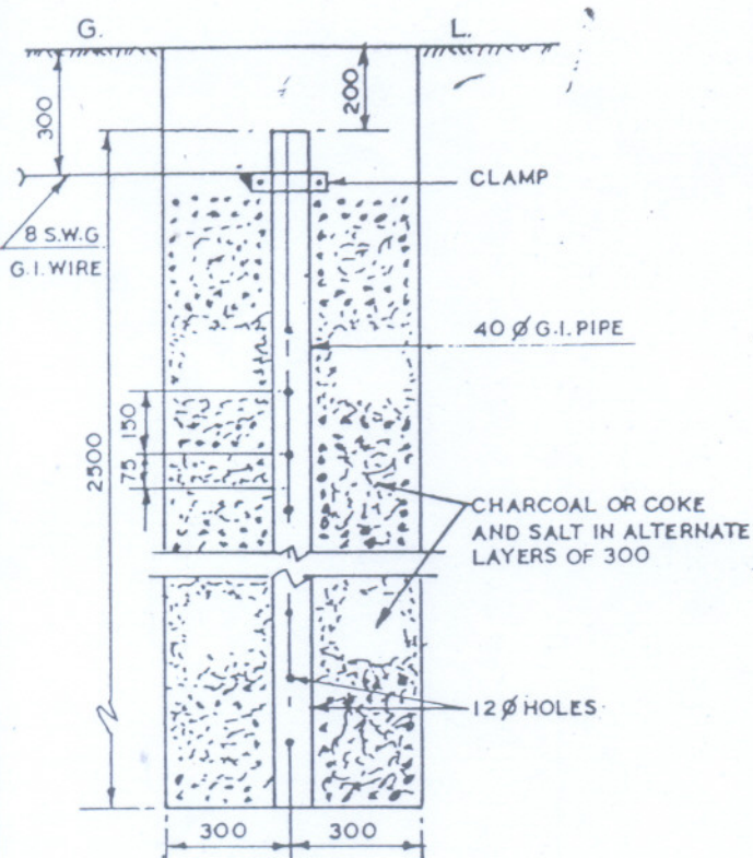
EARTHING FOR HARD, STIFF OR MEDIUM CLAY
