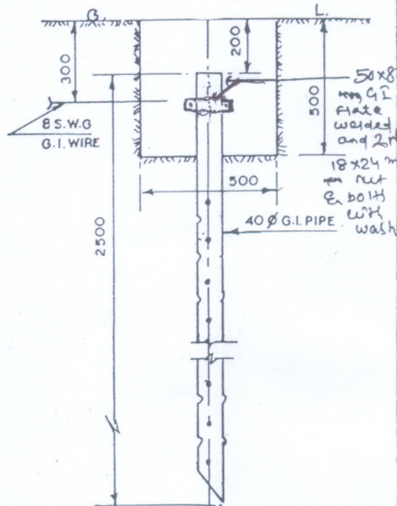
EARTHING FOR ORDINARY SOIL WHERE PIPE COULD BE HAMMERED IN
